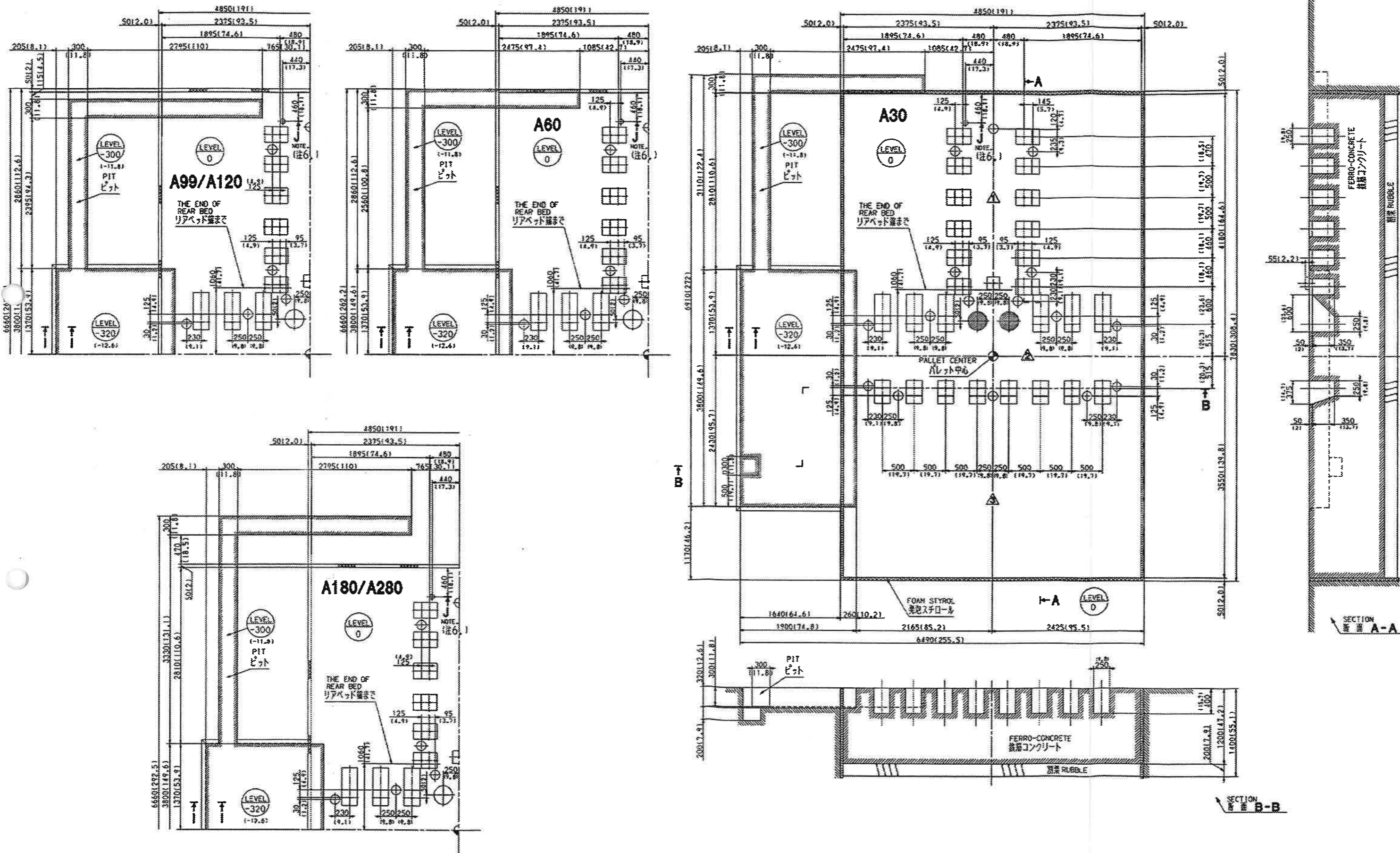
FIGURE 3-12 MACHINE FOUNDATION DIAGRAM (1)
